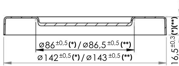
SECTION VIEW (SECTION A-A)
